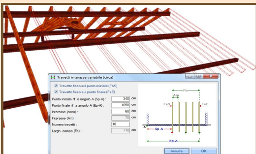
Free insertion of the struts
